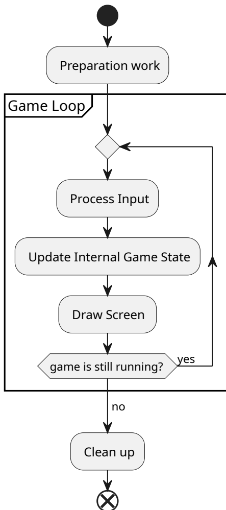
Figure 143: UML Diagram of the input-update-draw abstraction
